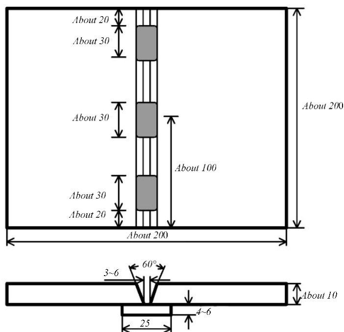
Fig. 9 Test piece P_{1tack} for tack butt welds
