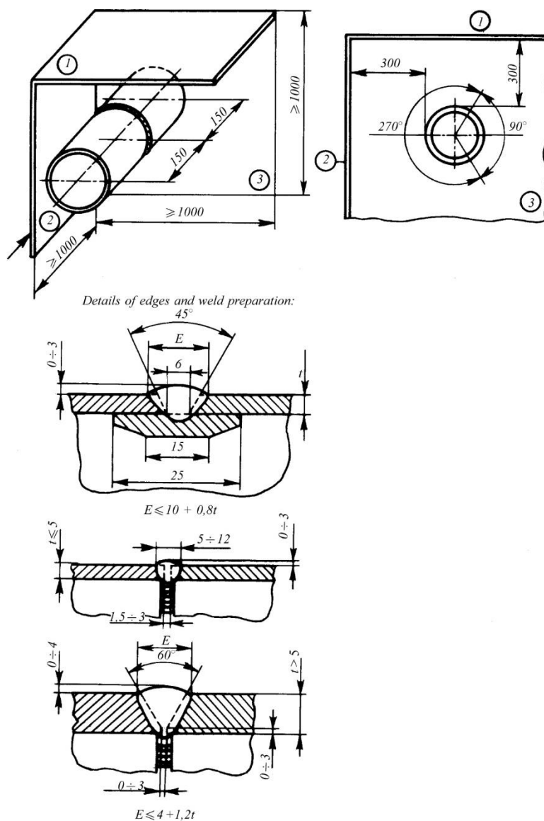
Test piece of pipe joint with a limited access to the welding zone P_5
