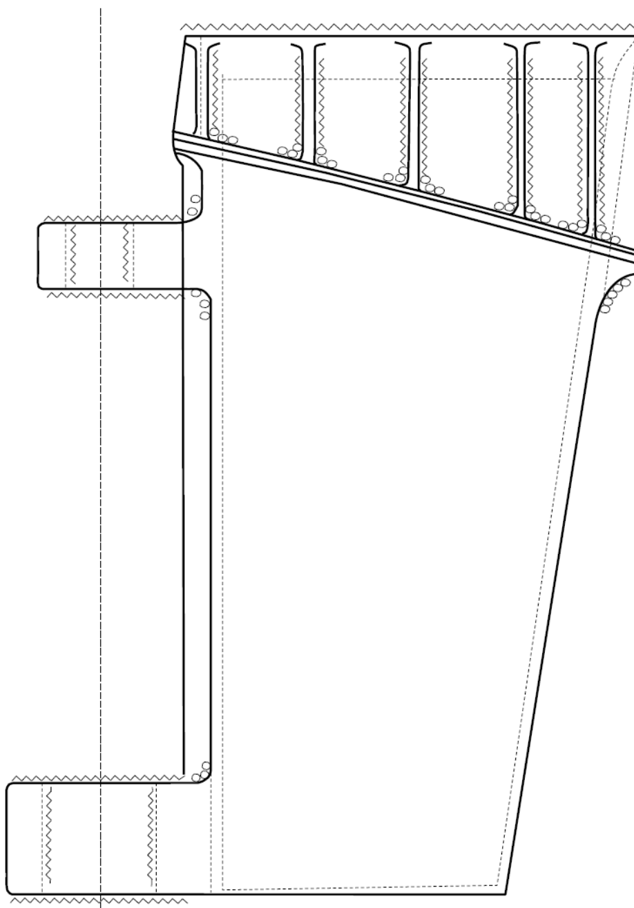
Fig. 2.5.2.4.1-4 Rudder hangings.
